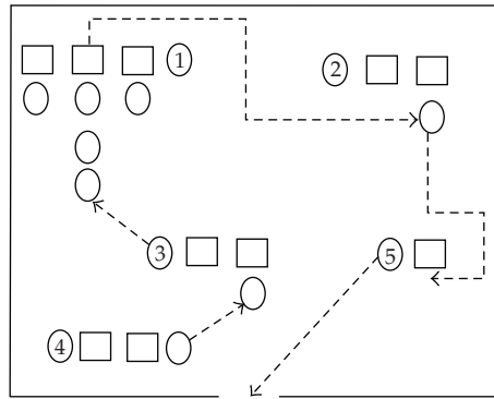
Figure 2: M/M/1 queues of the products/semiproducts in a job shop ( \square represents a server \circ represents a manufacturer of a semiproduct).
