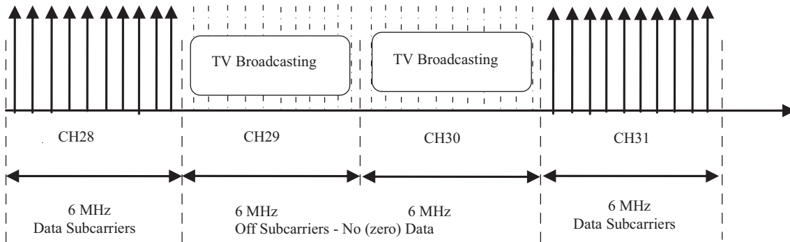
Figure 3. NC-OFDM within 4 consecutive channels.
