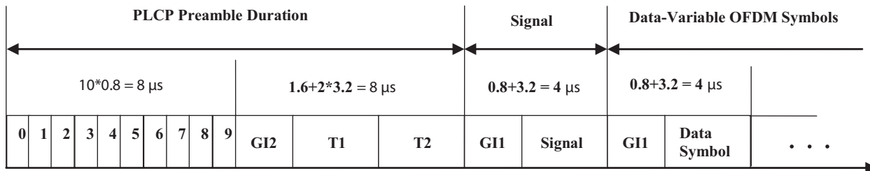
Figure 2. 802.11a physical layer frame format.
