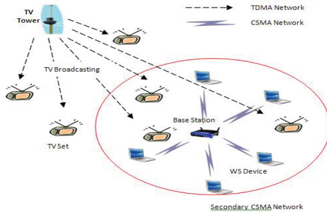
Figure 4. TDMA for primary network and CSMA for secondary network in TV bands.
